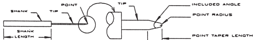
MODELE 407 CONFIGURATION ENLARGEMENT OF TIP
